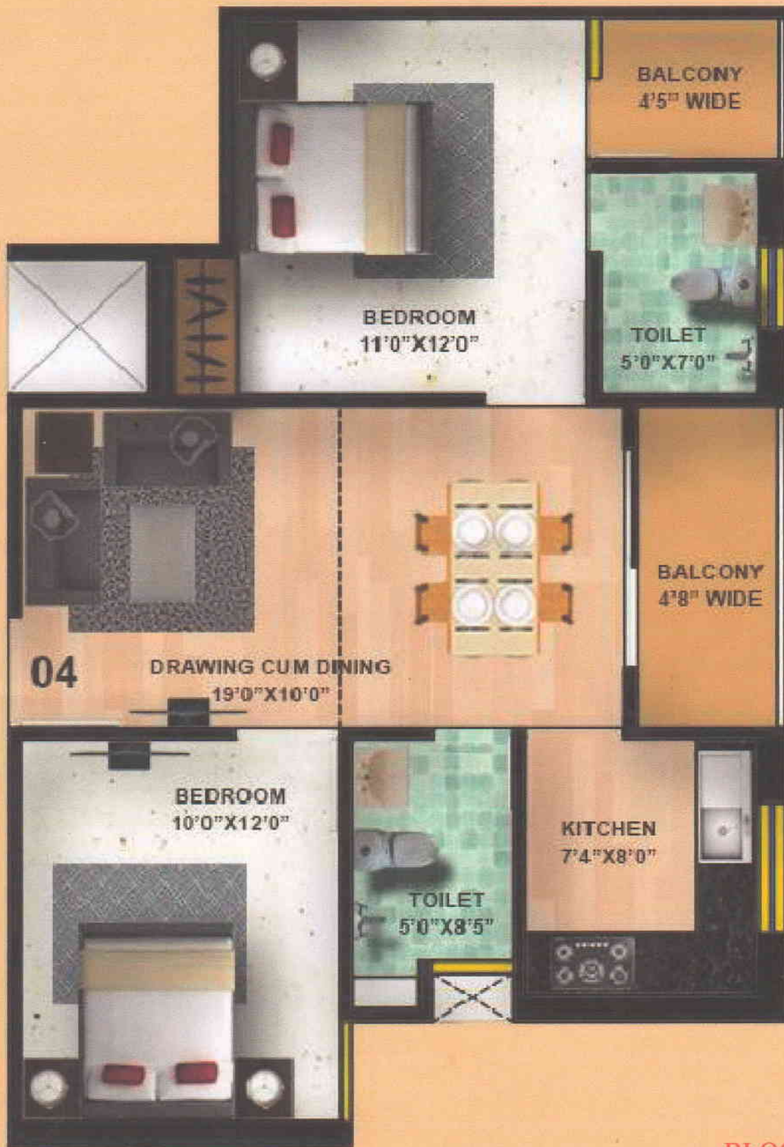
TYPICAL PLAN OF UNIT 4
